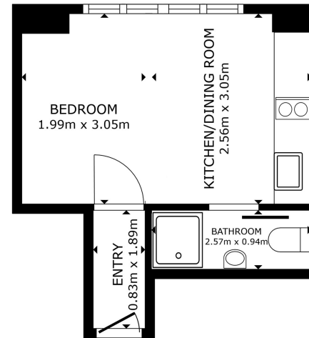
FLOOR PLAN
